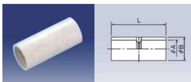
NDS-20, muffe
