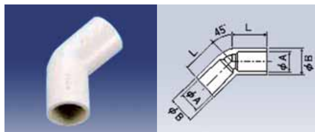
NDF-20, 45 grader
