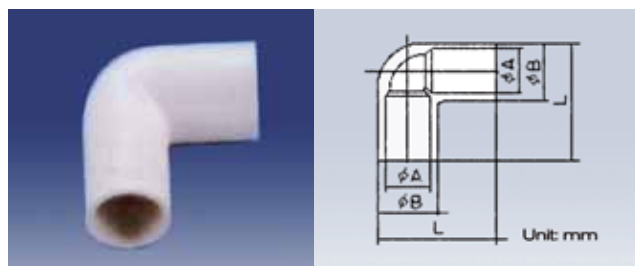
NDE-20, 90 grader
