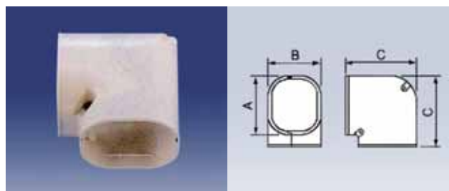
SKM, flat kort bend, 90 grader
