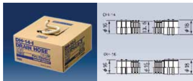
DH-14, DH-16
