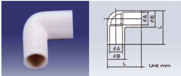
NDE-20, 90 grader
