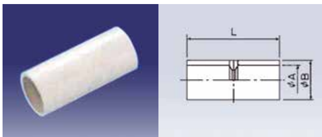
NDS-20, muffe
