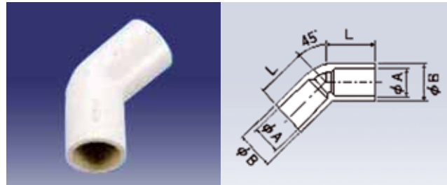
NDF-20, 45 grader
